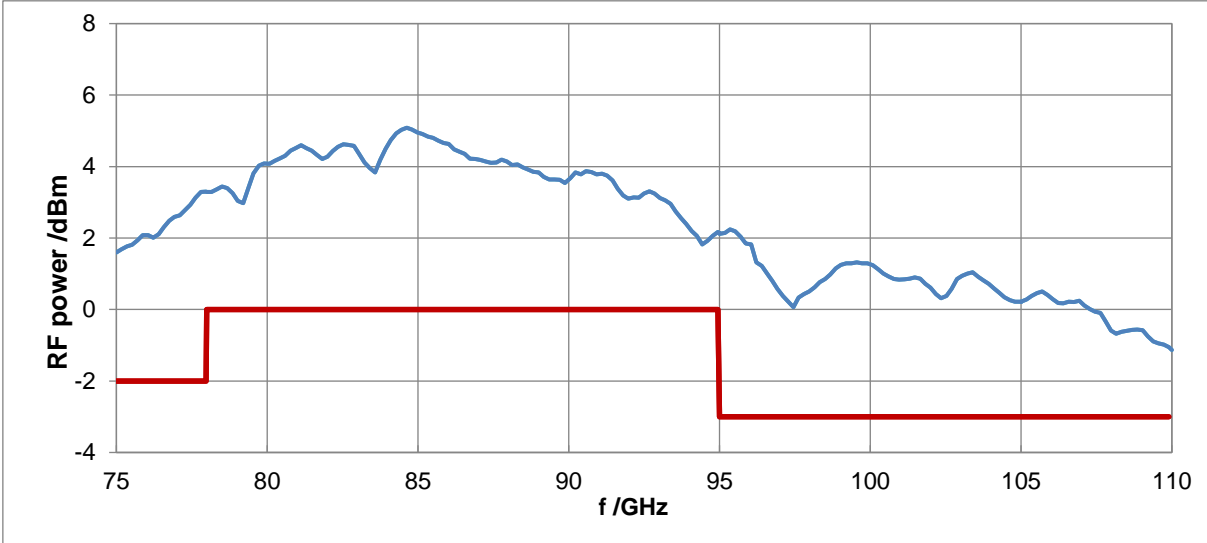
Test port output power versus frequency of the R&S®ZVA-Z110E (model .50)
