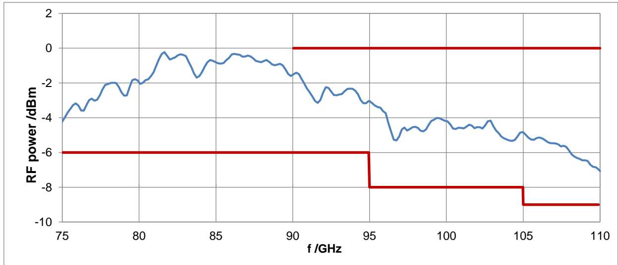
Test port output power versus frequency of the R&S®ZVA-Z110E (model .40)
